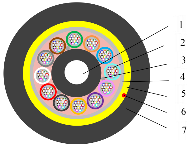
Cable Section Sketch Map
